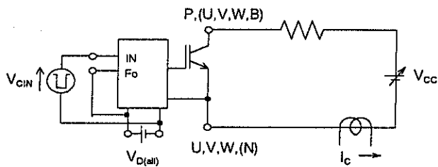
Fig.5 SC Test
